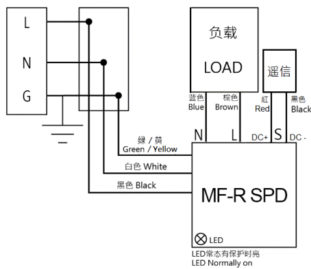
串联接法 Series Connection
