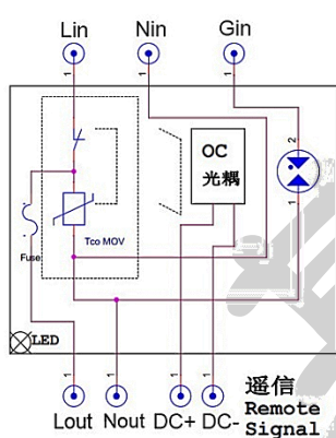
EZ10MF277M-S(C)-R
